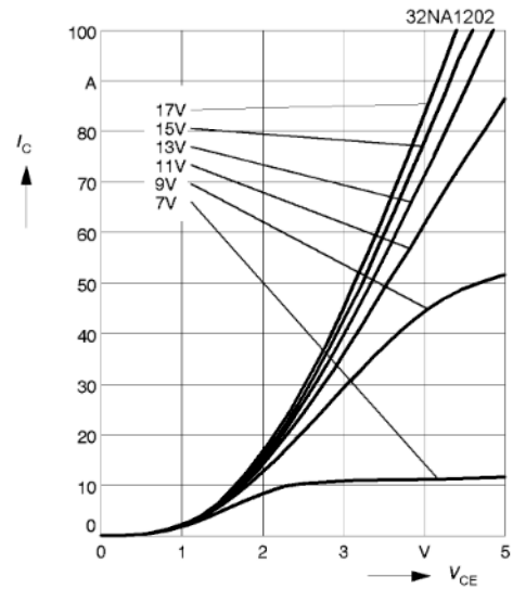
Fig. 2 Typ. output characteristic, t_p = 80 \text{ s} ; 125 \text{ }^\circ\text{C}
