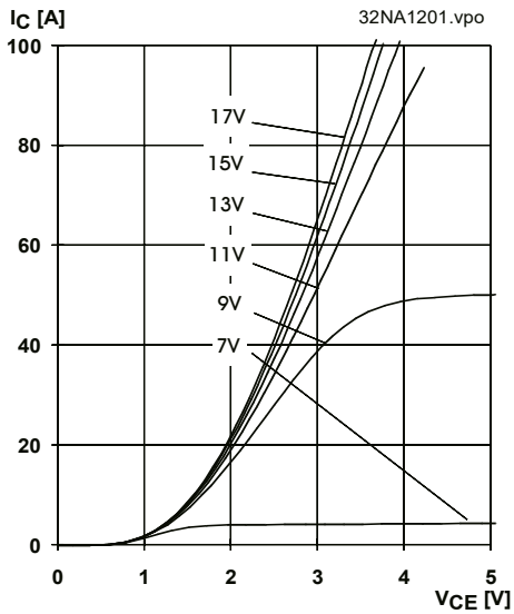
Fig. 1 Typ. output characteristic, t_p = 80 \text{ s} ; 25 \text{ }^\circ\text{C}
